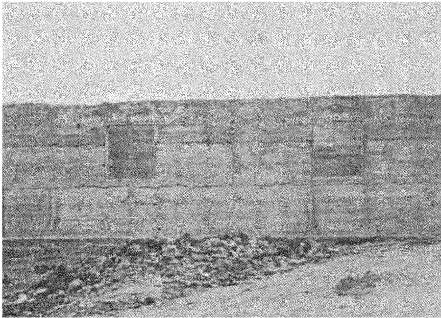
View of a whole wall tamped in three layers This wall has not yet been finished or water proofed. On top the rears that fix the wood tie beam to the earth wall can be seen.
